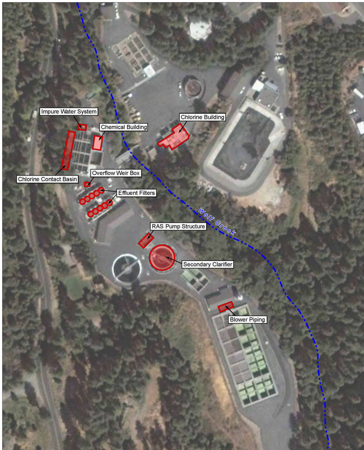
Figure 2: WWTP Project Elements
