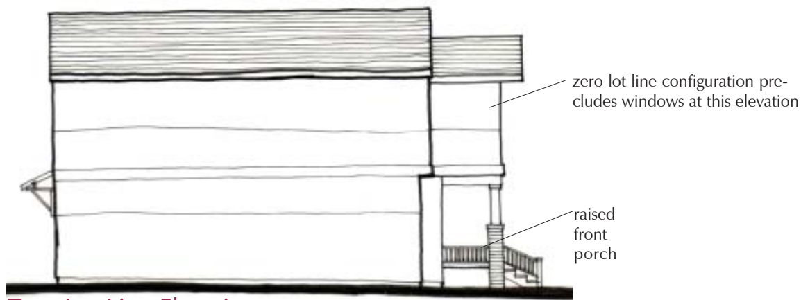
Zero Lot Line Elevation
